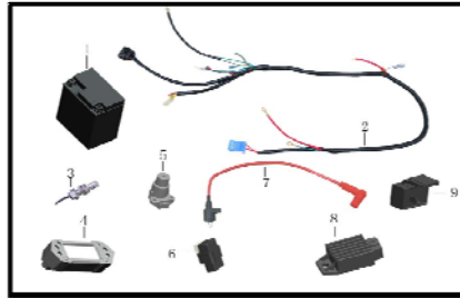
电零件 ELECTRICAL COMPONENTS . SECTION 12
