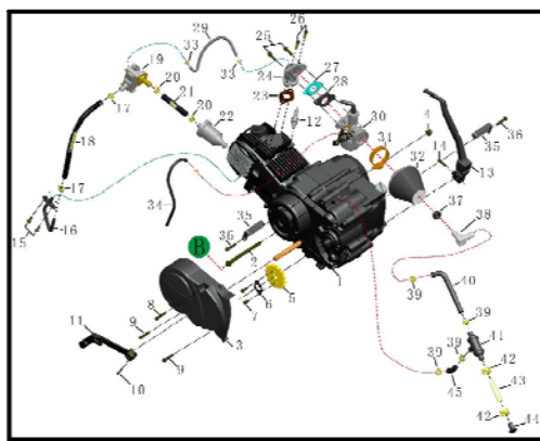
SECTION 1 发动机和化油器总成 ENGINE AND CARBURETOR ASSY.
