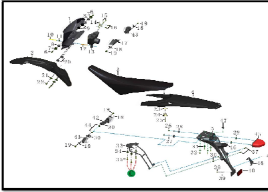
外罩总成/坐墊 FENDER AND SEAT ASSY. SECTION 10
