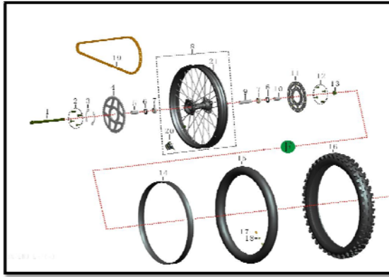
后轮总成 REAR WHEEL ASSY. SECTION 6
