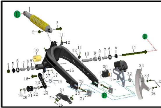
后平叉总成 REAR SWING ARM ASSY. SECTION 7
