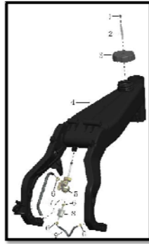
油箱总成 FUEL TANK ASSY. SECTION 11
