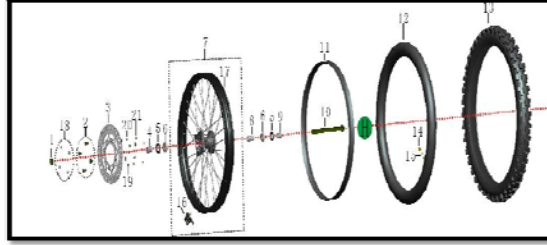
前轮总成 FRONT WHEEL ASSY. SECTION 5
